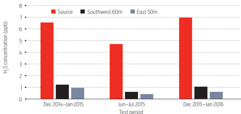
Figure 4. Averaged H 2 S concentration measured at three locations around a fumarole in Scion campus.
