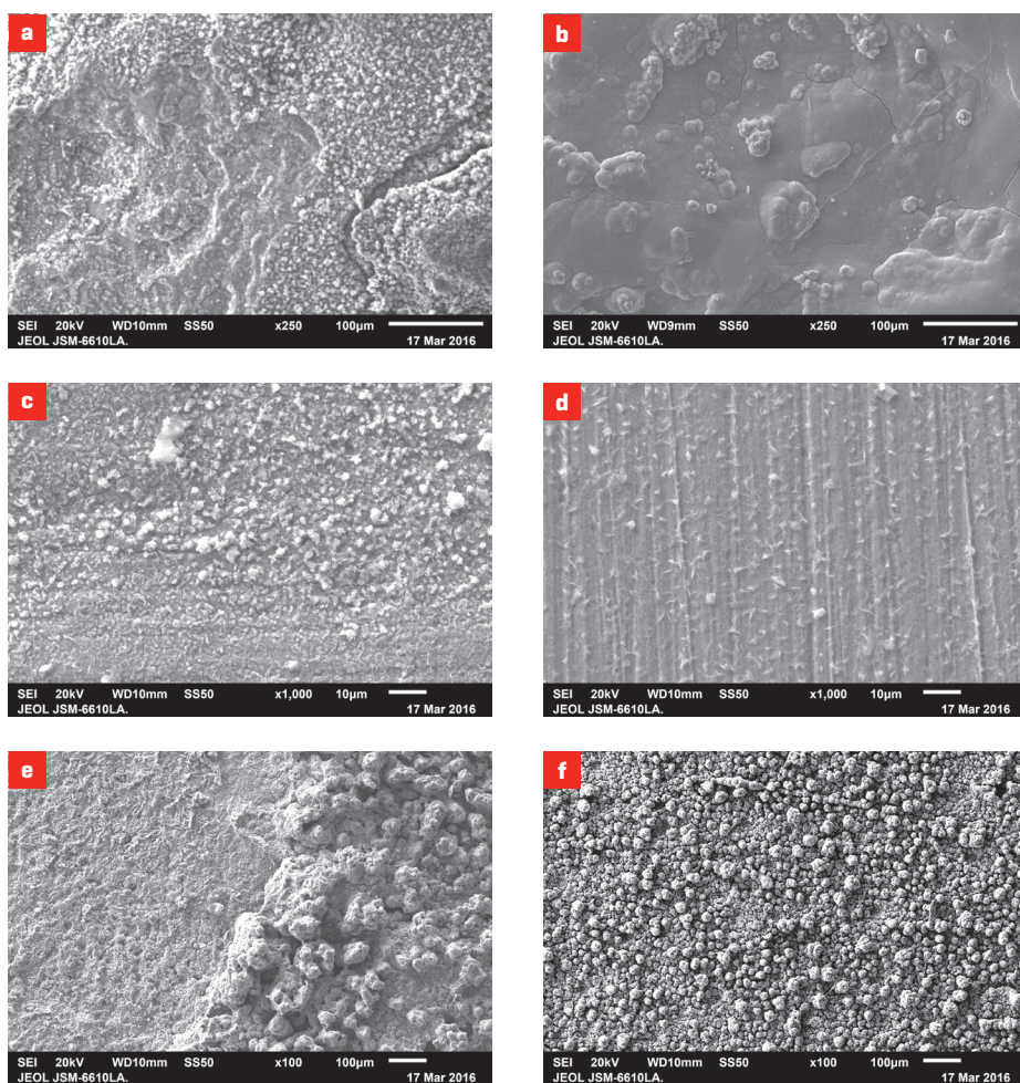
Figure 5. Surface of metal samples exposed for 1 year. a) Mild steel at 5 m from a fumarole. b) Mild steel at 50 m. c) Zinc at 5 m. d) Zinc at 50 m. e) Copper at 5 m. f) Copper at 50 m.
