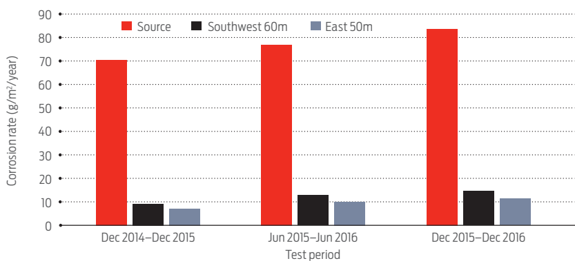
Figure 2. First-year corrosion rate of zinc exposed at three locations around a fumarole in Scion campus.
