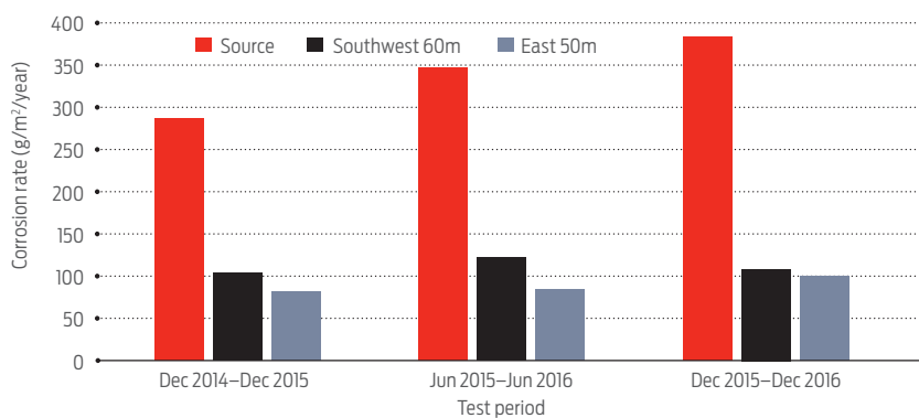
Figure 3. First-year corrosion rate of copper exposed at three locations around a fumarole in Scion campus.
