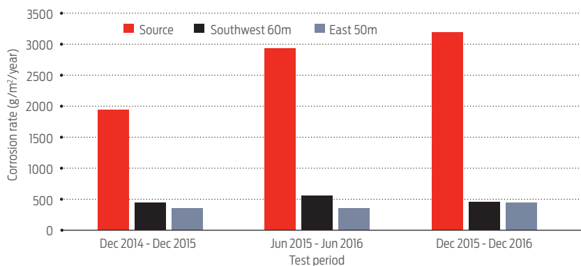
Figure 1. First-year corrosion rate of mild steel exposed at three locations around a fumarole in Scion campus.
