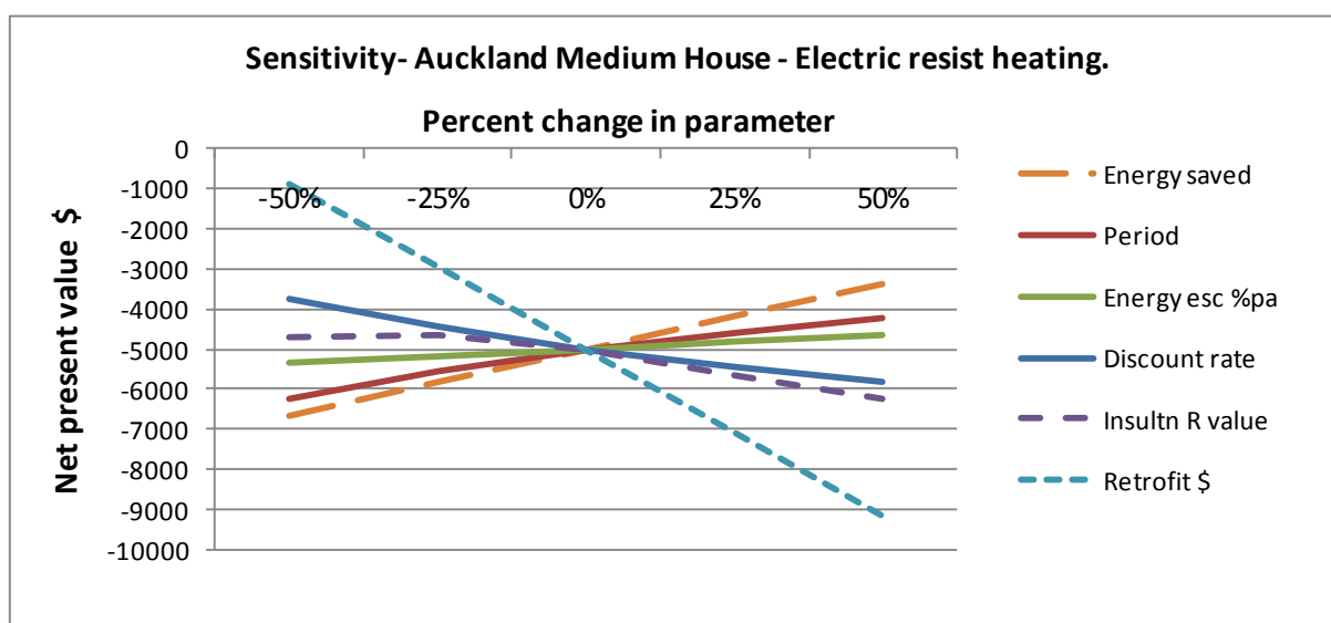
Figure 6. Sensitivity analysis – Auckland
