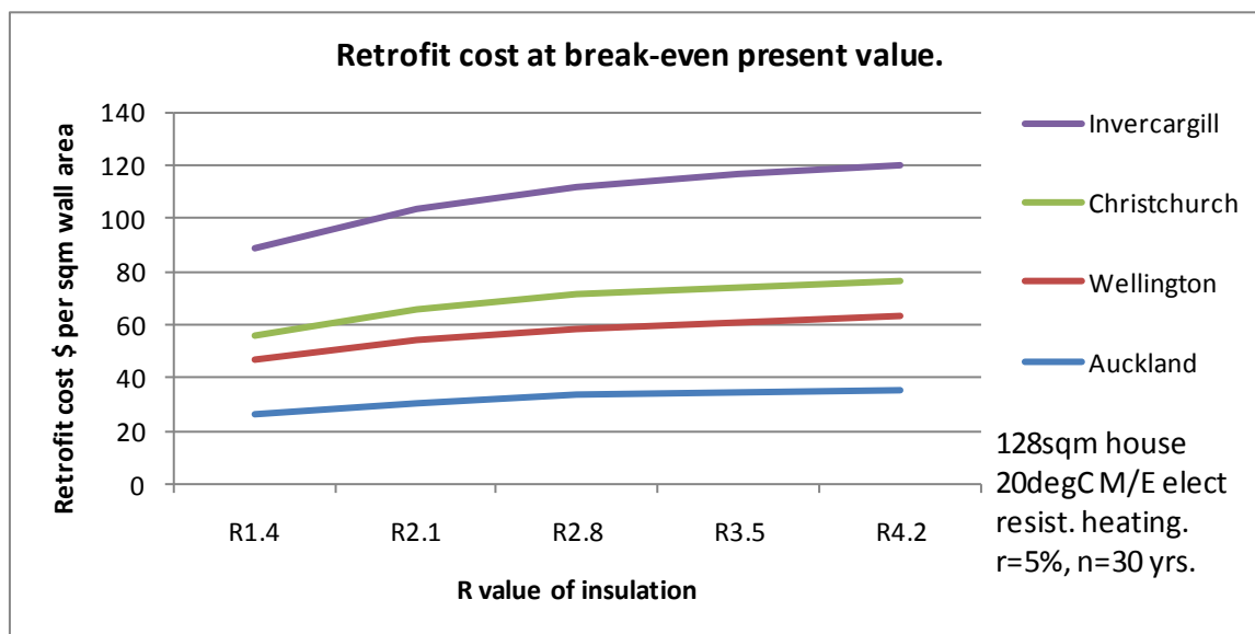
Figure 11. Required retrofit cost at break-even point by insulation R-value – default assumptions
