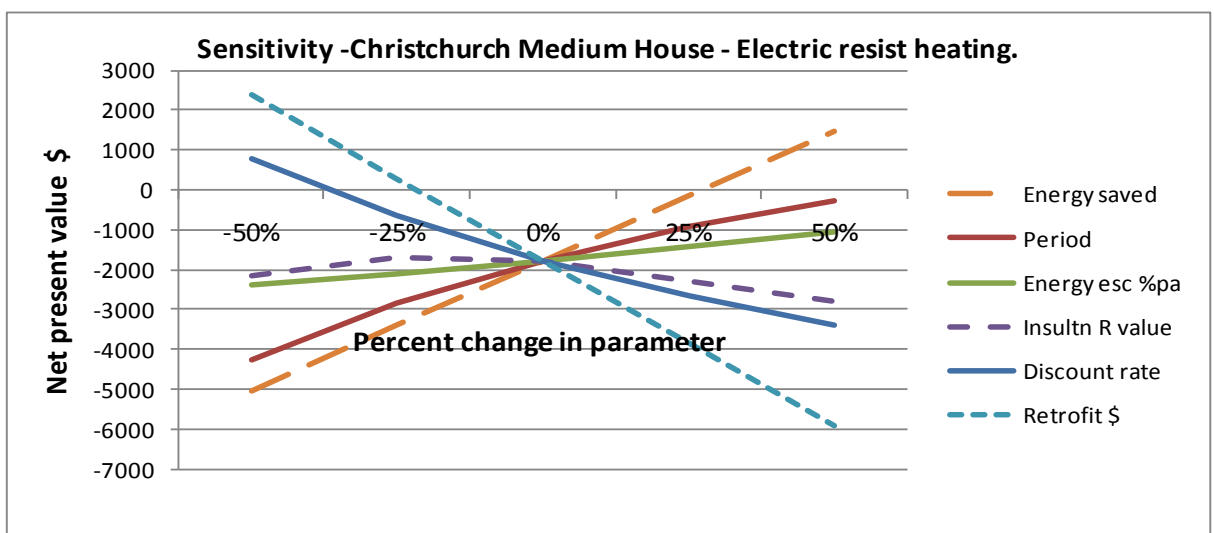
Figure 8. Sensitivity analysis – Christchurch
