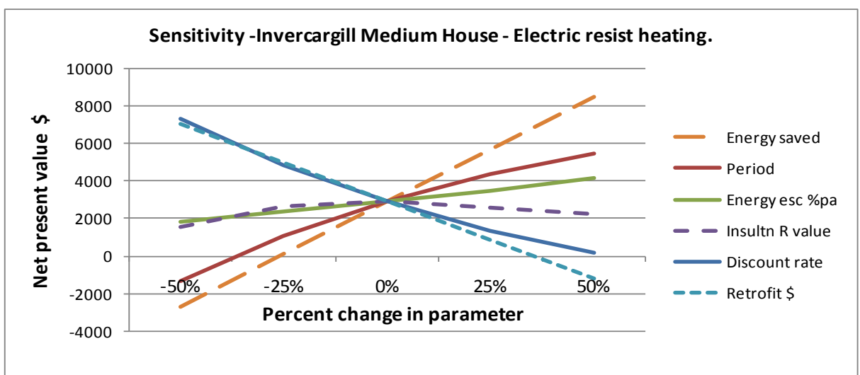
Figure 9. Sensitivity analysis – Invercargill
