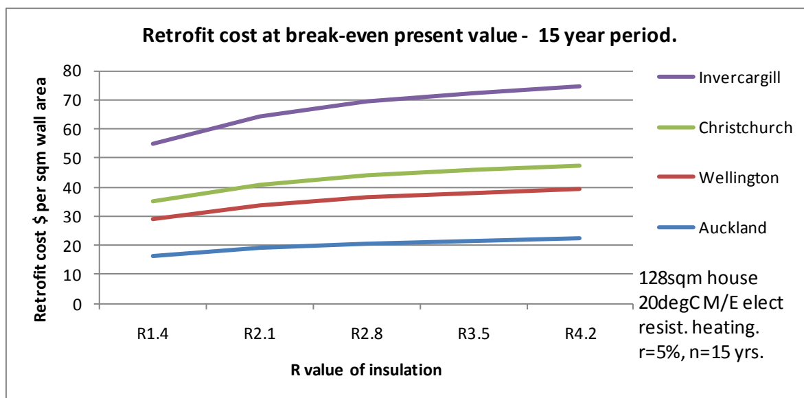
Figure 12. Required retrofit cost at break-even point by R-value – 15-year analysis period
