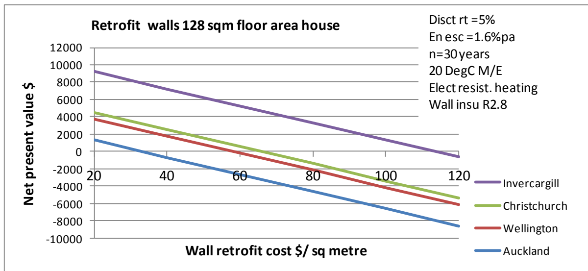
Figure 10. Wall retrofit cost and NPV
